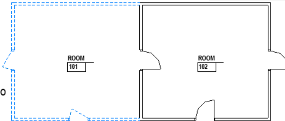
(A).FIRST FLOOR DEMOLITION PLAN
